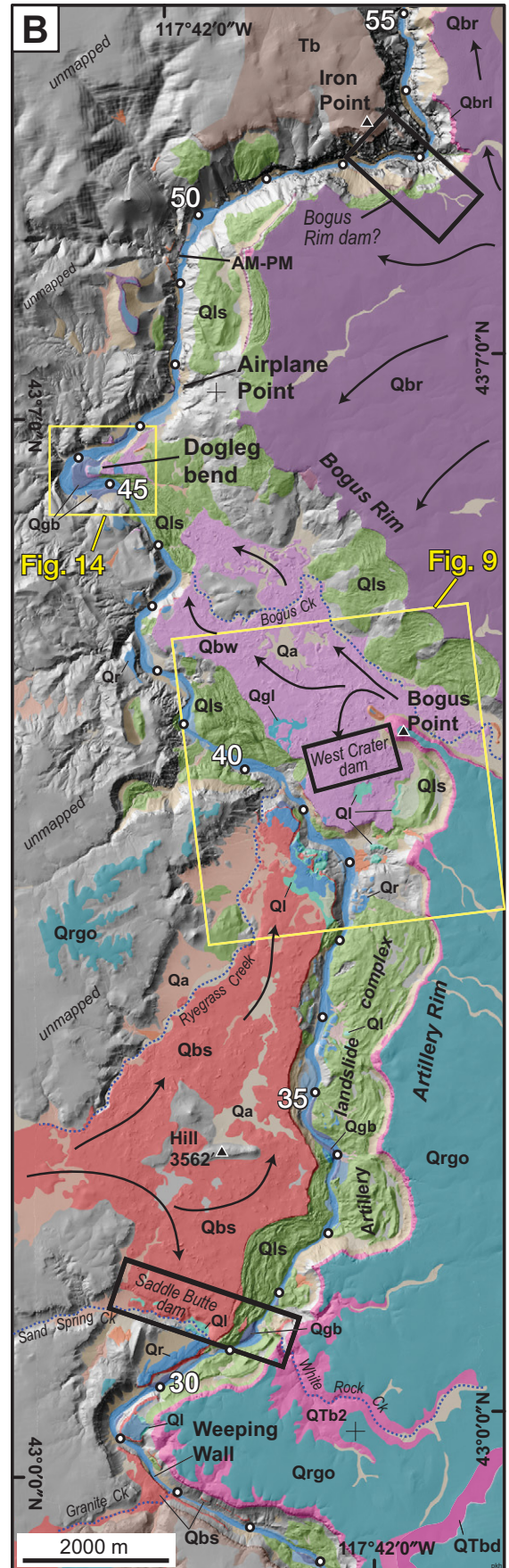
Figure 2. (A) General geologic map of the late Cenozoic lava flows and relevant geomorphic features of the Owyhee River study area. (B) Detailed geologic map of the upstream portion of the main study reach on a base map derived from a 1 m light detection and ranging (LiDAR) digital elevation model (DEM). Black rectangles mark the locations of the Bogus Rim, West Crater, and Saddle Butte lava dams. White numbers and circles along the river mark the river kilometers (Rk) downstream of the starting datum at Rome, Oregon (0 Rk). Yellow boxes outline areas of detailed maps in Figures 9 and 14.
