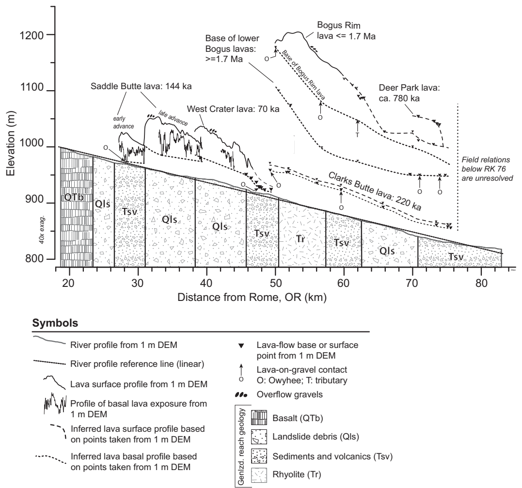
Figure 12. Longitudinal profiles of the Owyhee River and intracanyon lava flows from Rk 19 to 76. The lithologic units at the base of the diagram indicate the geologic units that compose the canyon walls at the river level in each reach. The narrow, bedrock canyon reaches are characterized by basalt (QTb) and rhyolite (Tr) bedrock, and the wider reaches are dominated by sediment interbedded with thin volcanic layers (Tsv) or landslide debris (Qls). The surface of the West Crater flow markedly steepens as it approaches the bedrock gorge at Rk 46. Arrows indicate locations where the lava directly overlies river gravels (O) or tributary gravels (T), which most closely represent the paleo-river channel elevations. The dotted lines approximate the paleo-valley gradients based on the basal contacts of the lava flows. The basal profiles of the lower Bogus and Bogus Rim lava flows portray a valley gradient significantly steeper than today through the rhyolite gorge. The paleochannel profile preserved by the strath terraces overlain by remnants of the Clarks Butte lava is only slightly steeper than that of the modern river.
